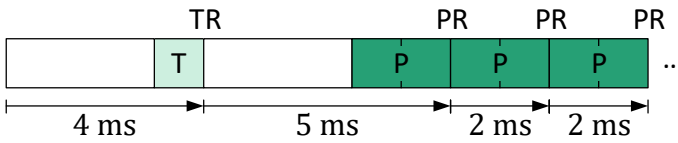
Figure 8: Typical timings for a continuous pressure-only measurement ( MEAS\_T = 0 , P\_CONV = 0 ) with activated 2× oversampling ( OVSP = 1 )
