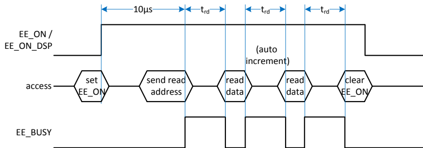
Figure 4-9 EEPROM power controlled automatically: Write/ Erase/ Block write/ Block erase
