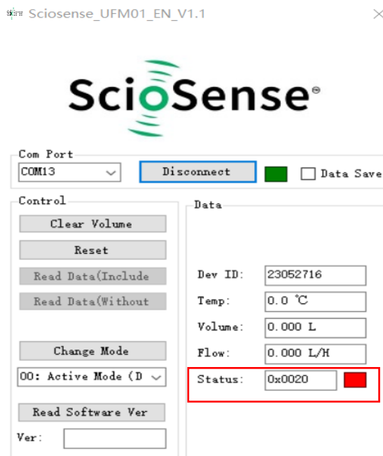
Figure 7: Status Error
